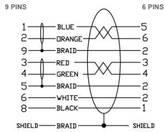
PINOUT 9 TO 6 FIREWIRE CABLE
