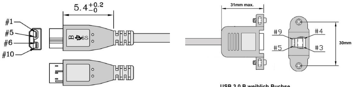
USB 3.0 B weiblich Buchse USB 3.0 B female USB 3.0 B femelle
