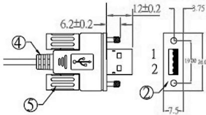
USB 2.0 A plug A100-547-001
