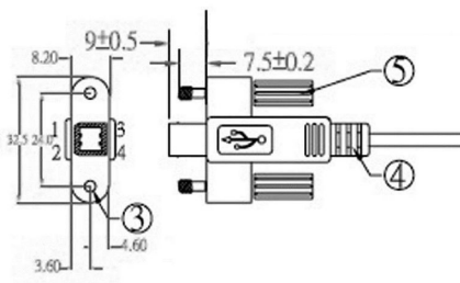
USB 2.0 B plug A110-507-001
